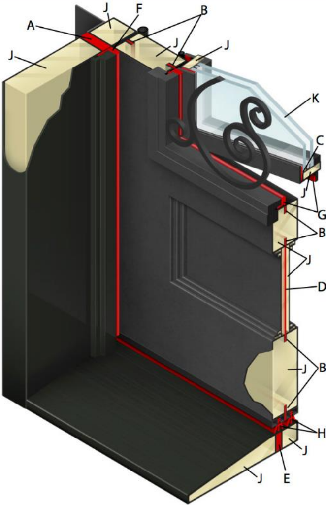
Conduction Causes 90% of Heat Loss Through an Iron Door
